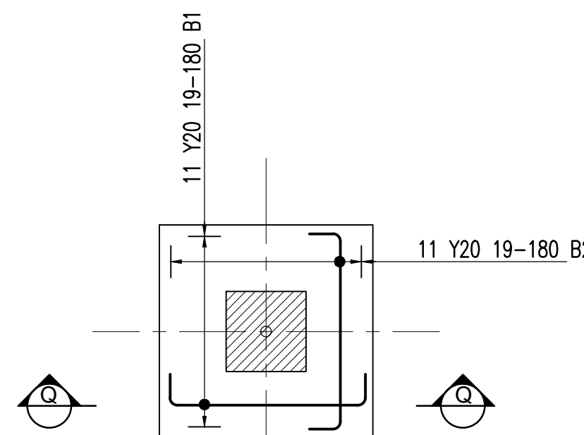
BASE TYPE (N) 2000x2000x1000 THK. COLUMN: 750x750 S12/45, S12/43, S11/45 & S11/43
