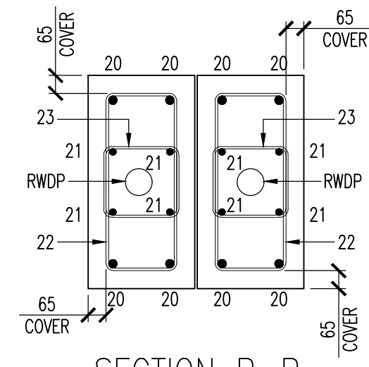
SECTION P-P
