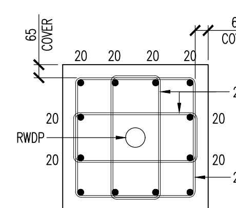
SECTION R-R
