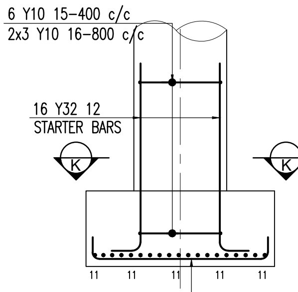
SECTION J-J
