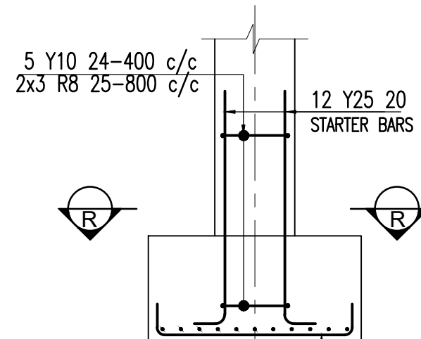
SECTION Q-Q
