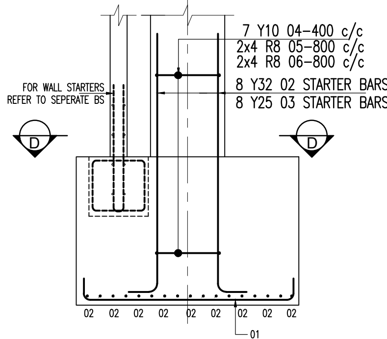
SECTION C-C
