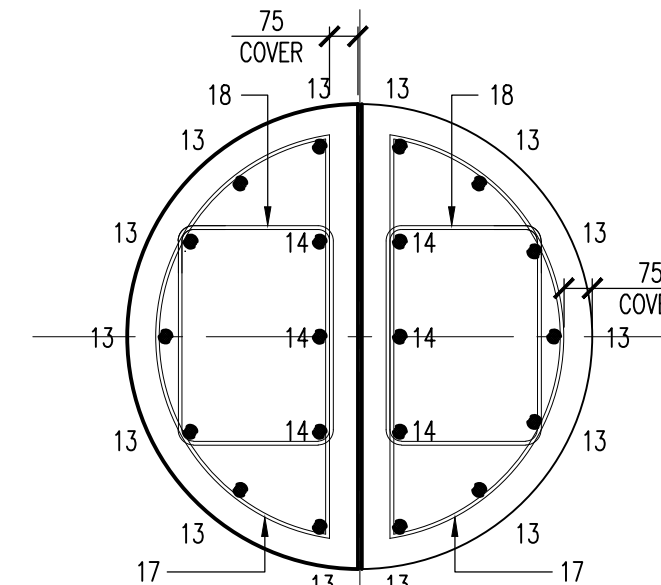
SECTION M-M
