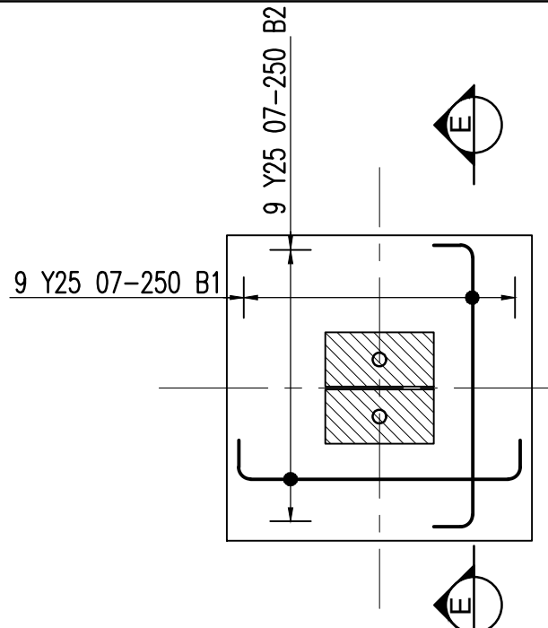
BASE TYPE (M) 2250x2250x1000 THK. COLUMNS: 2/400x800 S10/45a-45b & S10/43a-43b
