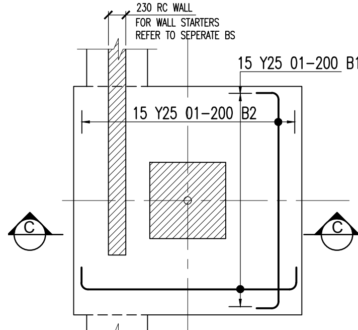
BASE TYPE (F) 3000x3000x2000 THK. COLUMN: 1000x1000 S12/53
