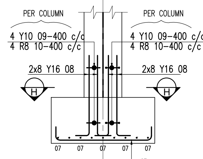
SECTION G-G
