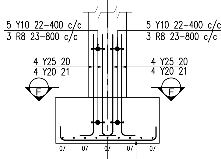
SECTION E-E
