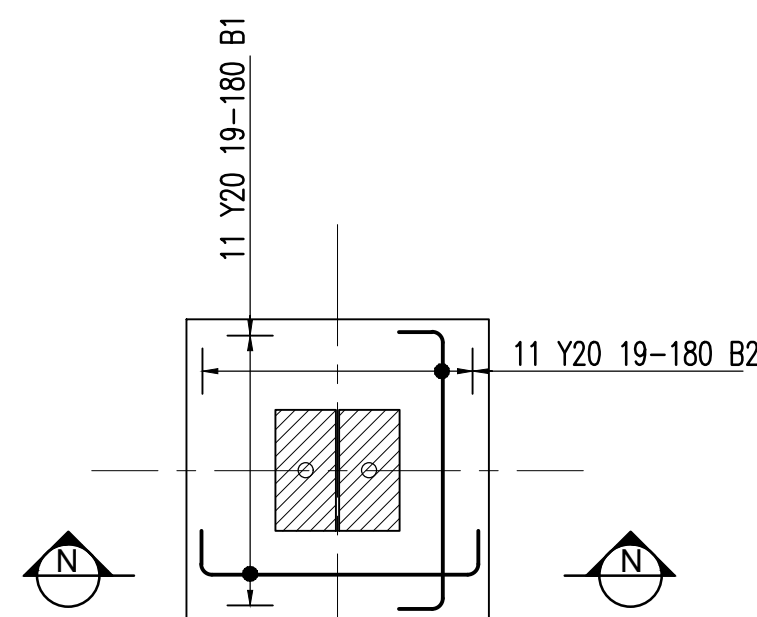
BASE TYPE (N) 2000x2000x1000 THK. DOUBLE COLUMNS: 2/400x800 S12/41a-41b & S11/41a-41b
