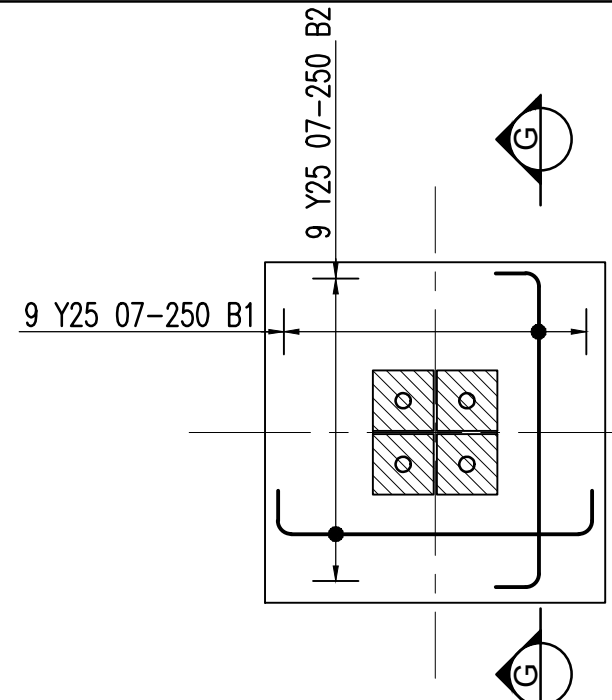
BASE TYPE (M) 2250x2250x1000 THK. COLUMNS: 4/400x400 S10/41a-41b-41c-41d
