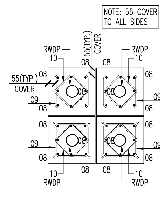
SECTION H-H
