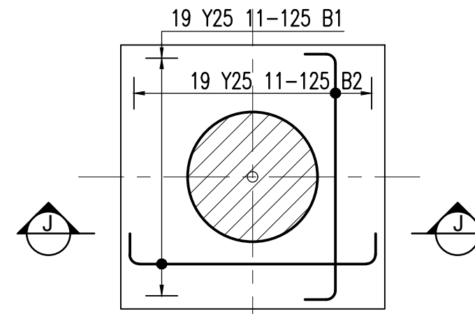
BASE TYPE (L) 3750x3750x1000 COLUMN: 1260Ø S14/45, S14/43, S13/45 & S13/43
