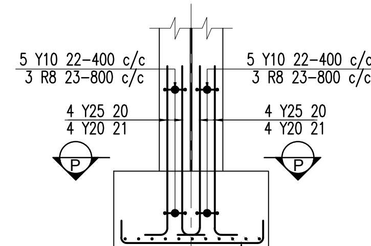
SECTION N-N
