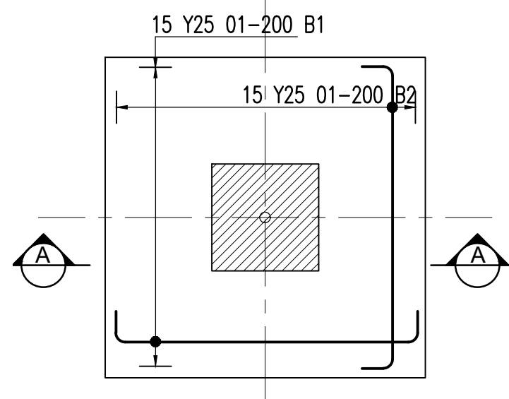
BASE TYPE (F) 3000x3000x2000 THK. COLUMN: 1000x1000 S12/47
