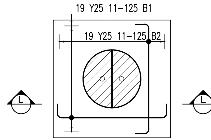
BASE TYPE (L) 3750x3750x1000 2/ HALF ROUND COLUMNS: 1260Ø S14/41a-41b & S13/41a-41b
