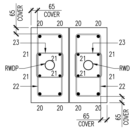
SECTION F-F
