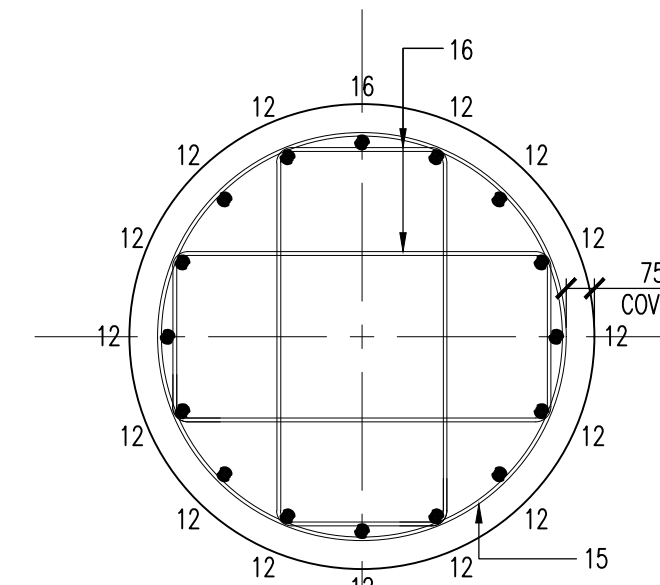
SECTION K-K
